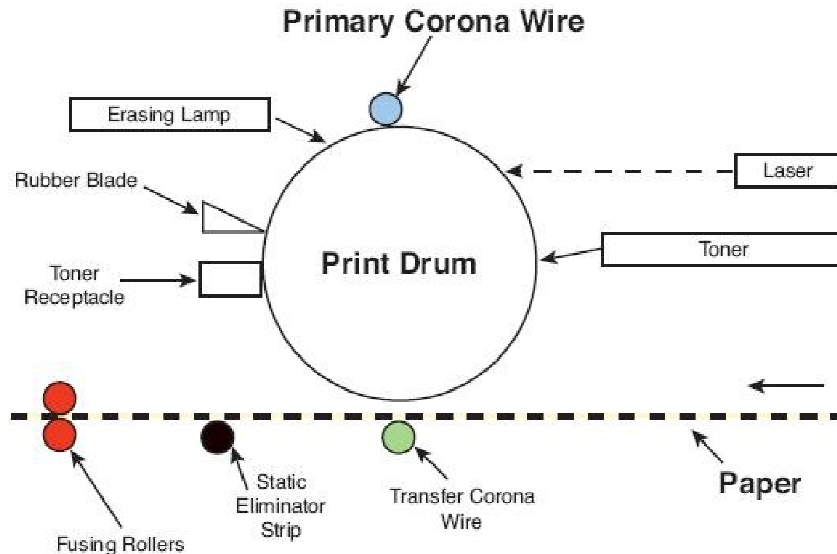
Components involved in the six-step laser printing process
